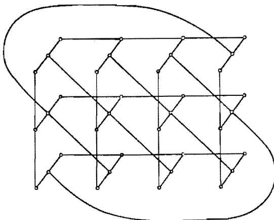
FIGURE 11. G_{3,4}
