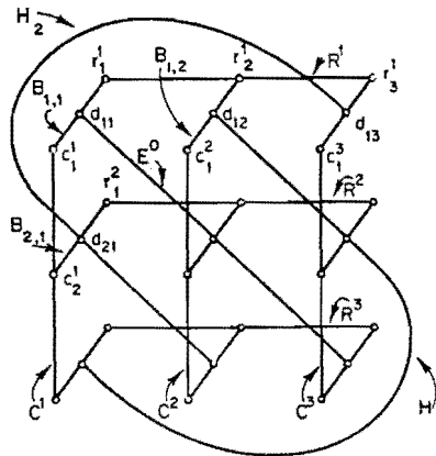
FIGURE 10. G_{3,3}
