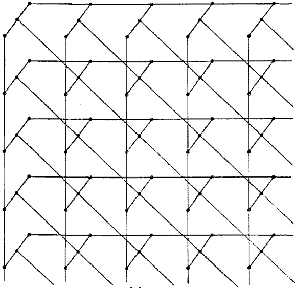
FIGURE 12. G_{\infty, \infty}
