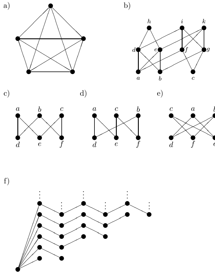
Figure 1.1: a) The complete graph with 5 vertices K_5 , b) The diagram of an ordered set (the set P2 in [234]), c)-e) Three diagrams for the same ordered set (points to be identified by an isomorphism have the same letters), f) The “diagram” of an infinite ordered set (this “spider”, as Rutkowski named it, is taken from [267], Remark 5.1).
