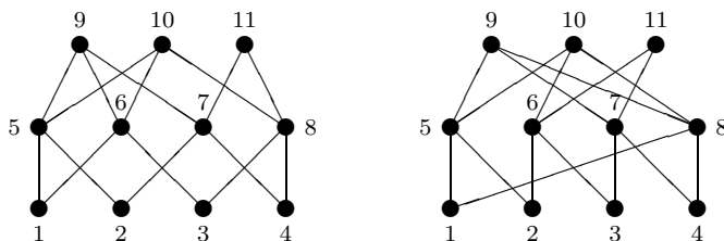
Figure 1.3: Two isomorphic ordered sets.
